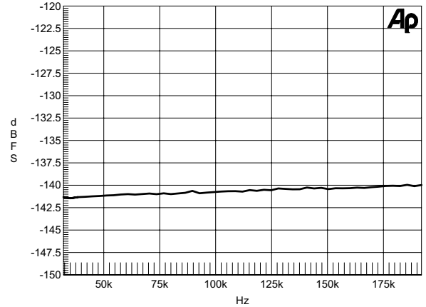
Figure 38. THD+N vs. Output Sample Rate, 0 dBFS 1 kHz Tone, Fsi = 192 kHz
