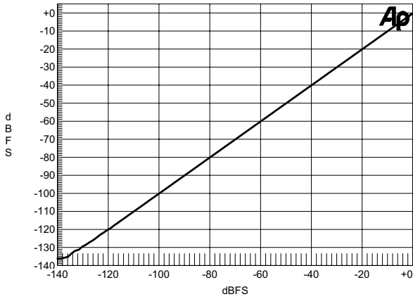
Figure 51. Linearity Error, 0 to -140 dBFS Input, 200 Hz Tone, 48 kHz:44.1 kHz
