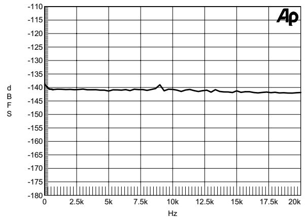
Figure 66. THD+N vs. Frequency Input, 0 dBFS, 96 kHz:48 kHz
